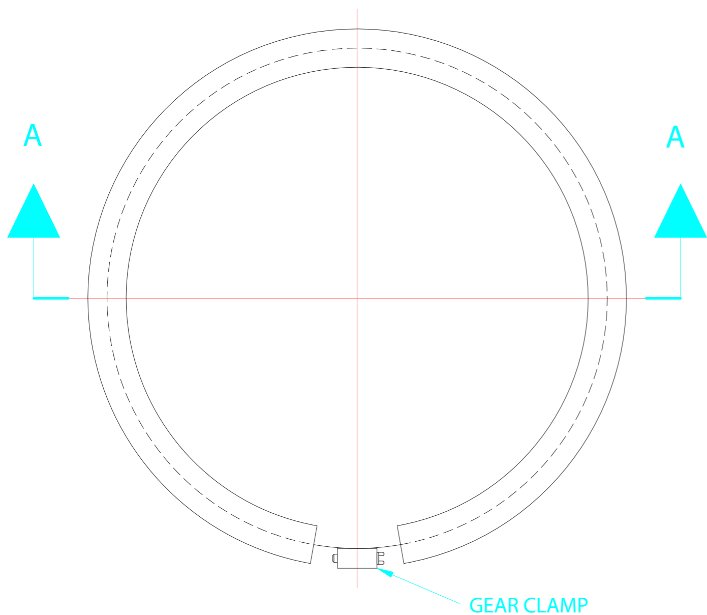
PLAN
